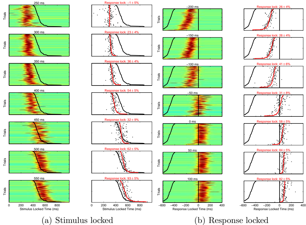
Fig. 5. Detailed temporal analysis of stimulus locked (a) and response locked (b) discriminating activity for subject 2. Each row in the left column shows the fit of discriminating activity from Figure 3 to a Gaussian profile described by Equation 8. On the top of each of these panels is the onset time of the window used for discrimination. Right columns of each panel display the peak latency ( \mu ) (black dots) of each trial. The projection of response times onto these peak latencies is shown with a red curve (stimulus times were projected onto peak latencies for the response locked condition). The parameters for this projection indicate the degree of response locking for each component. Purely stimulus and response locked conditions are indicated by 0% and 100% response lock respectively. On top of these panels are reported the percent response lock and corresponding error in the fit of the peak latencies across trials as well as the mean onset time of the component. The standard deviation of peak latencies is 62 ms for stimulus locked and 66 ms for response locked results shown.
