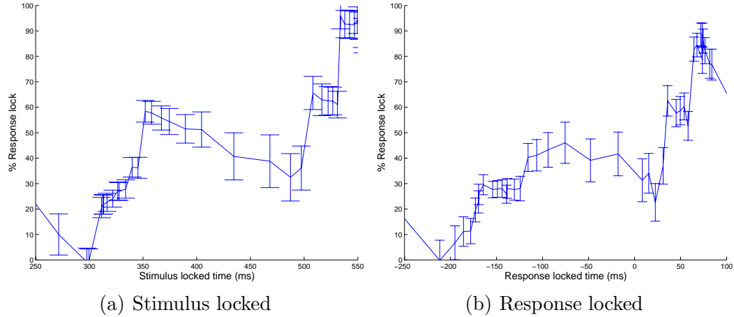
Fig. 6. Degree of response locking over time derived from stimulus (a) and response locked (b) discriminating components for subject 2. Response lock %'s are from projections shown in Figure 5. Error bars reflect standard error of the regression parameter associated with response locking %.
