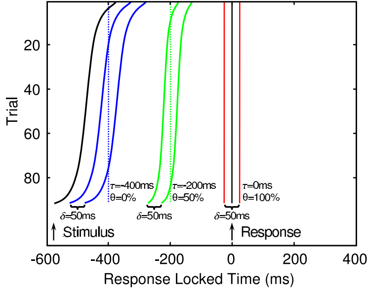
Fig. 2. Parameters of the training window defined for logistic regression (Equation 3). We define a training window starting at a relative onset time \tau , with a duration of \delta and orientation \theta (relative to response time). Shown are three examples of training windows with \tau = -400ms, \theta = 0\% (blue sigmoids), \tau = -200ms, \theta = 50\% (green sigmoids) and \tau = 0ms, \theta = 100\% (red vertical lines). The duration of all training windows is \delta = 50ms .
