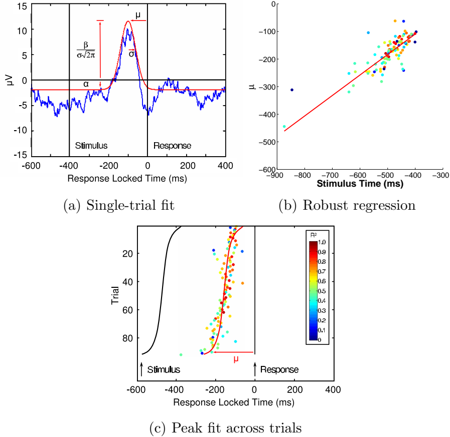
Fig. 4. Illustration of single-trial fitting procedure and estimation of percent response locking. (a) Fit \hat{y}(t) (Equation 8) for component activity y_c(t) (Equation 3) for one trial. Parameters of single-trial fit: \mu corresponds to discriminating component peak latency relative to the response and \sigma loosely indicates component duration. (b) Robust regression of component latencies \mu and response times r as described by Equation 9 for Subject 2, response locked \tau = -200ms . Predicted \hat{\mu} is shown by the red line. In response locked analysis, stimulus time ( -r ) is used in the regression rather than response time r . For response locked analysis, the degree of response locking is then defined as 1 - \theta rather than \theta as in stimulus locked analysis. Subtracting the slope of the red line ( \hat{\mu} ) from one corresponds to the degree of response locking shown in Figures 5(b)– 8(b). (c) Displaying the fit from this regression across trials helps to visualize the degree of response locking. Component peak latencies \mu across trials are shown by colored dots. The color of the peaks corresponds to the R^2 value indicating the goodness-of-fit for \hat{y}(t) . Note that points with a large R^2 tend to lie along the fitted curve. Stimulus onset time (black sigmoid) is fit to peak latencies to quantify degree of component response locking across trials (red sigmoid)
