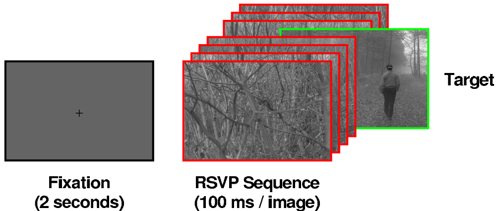
Fig. 1. Example Rapid Serial Visual Presentation (RSVP) trial. A fixation cross lasting two seconds is followed by a sequence of 50 images. Each sequence has a 50% probability of containing one target image. This target can only appear within the middle 30 images to ensure that a one second image buffer precedes and follows the target.
