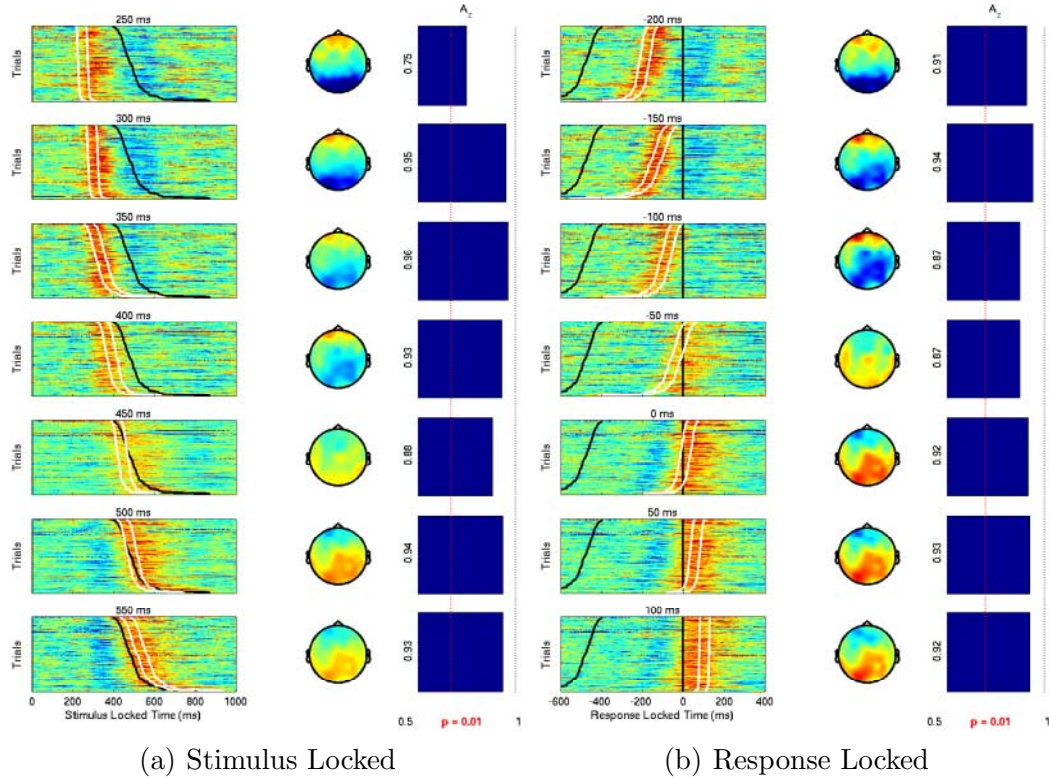
Fig. 3. Discriminating component activity shows the difference between target and non-target trials. Stimulus locked (a) and response locked (b) component activity y (Equation 3) for subject 2. The activity is color coded (positive activity is red, negative activity is blue). Trials are sorted by response time and aligned vertically so that stimulus or button release time is at 0 ms for stimulus or response locked panels respectively (vertical black line). The black “S”-shaped curve indicates the response or stimulus for stimulus or response locked plots respectively. Each row shows the activity extracted for a window of \delta = 50 ms duration. The beginning and end of this window is displayed with two white curves. The profile (i.e. orientation \theta ) of this window is derived by scaling response times across trials. The degree of scaling was determined by searching for the scaled training window yielding maximum discrimination performance. Moving the window by varying \tau , enables discriminating activity for various latencies to be extracted. A representation of the topology of the extracted activity (Equation 7) is shown to the right (dorsal view). The color code indicates (red) positive correlation of the sensor readings with the extracted activity and (blue) negative correlation. These scalp plots can be thought of as a coupling of the discriminating activity with the sensors, reflecting the proximity and orientation of the discriminating activity. The A_z value shown as a bar graph indicates the significance of the differential activity. The red dotted line corresponds to p = 0.01 .
